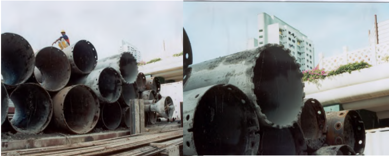
Double Wall Casings (for secant pile wall)
